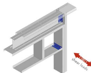
Head-to-Jamb Connections
