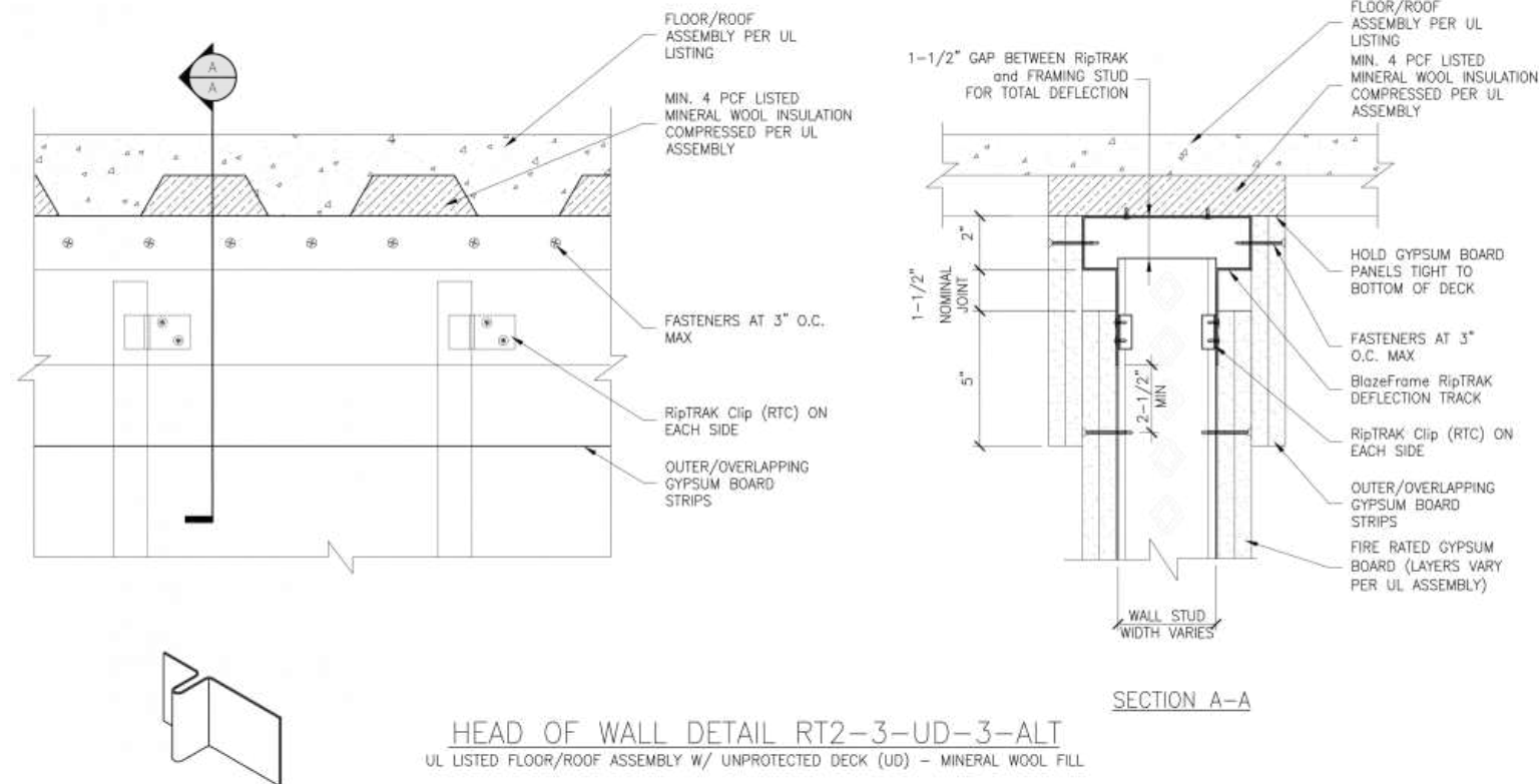
UL DESIGN HW-D-1125 (ALT 3A1 and 3B1) (2 HR WITH 1-1/2" NOMINAL JOINT)
