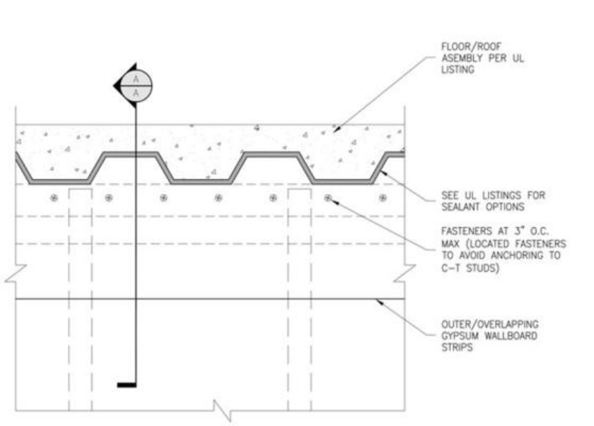
HEAD OF WALL DETAIL SWRT1-1-UD-1 UL LISTED FLOOR/ROOF ASSEMBLY W/ UNPROTECTED DECK (UD) - MINERAL WOOL FILL
