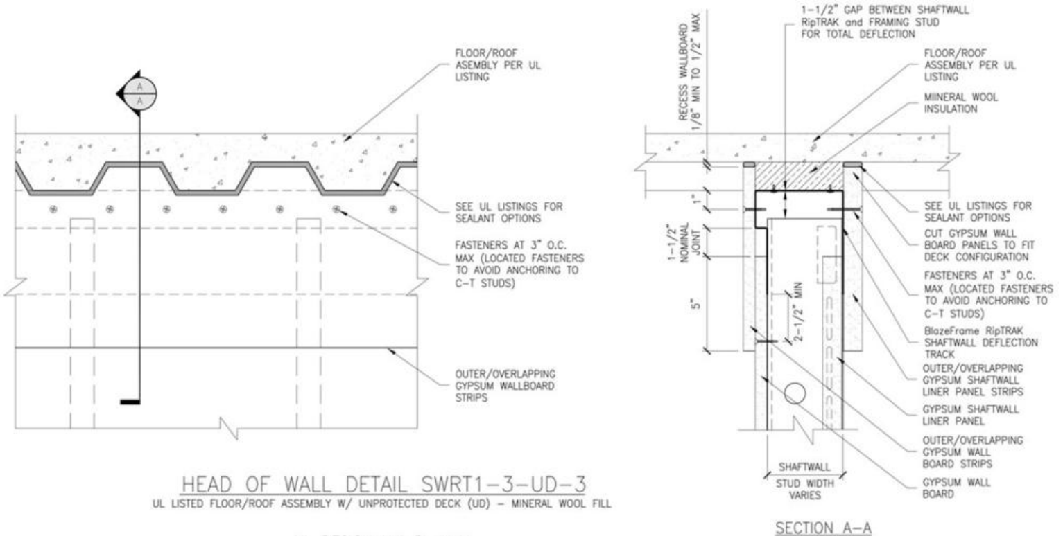
UL DESIGN HW-D-1141 (1 HR WITH 1-1/2" NOMINAL JOINT)
