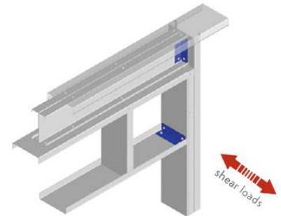
Head-to-Jamb Connections
