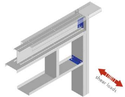
Head-to-Jamb Connections
