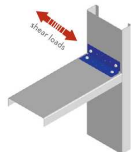
Sill-to-Jamb Connections
