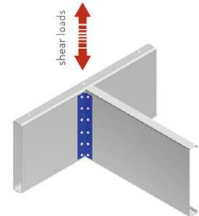
Joist-to-Joist Connections
