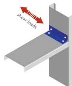
Sill-to-Jamb Connections
