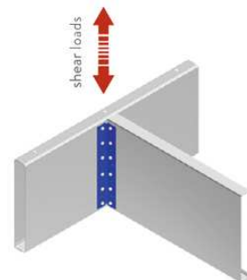
Joist-to-Joist Connections
