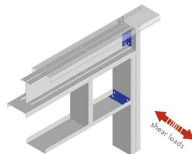
Head-to-Jamb Connections
